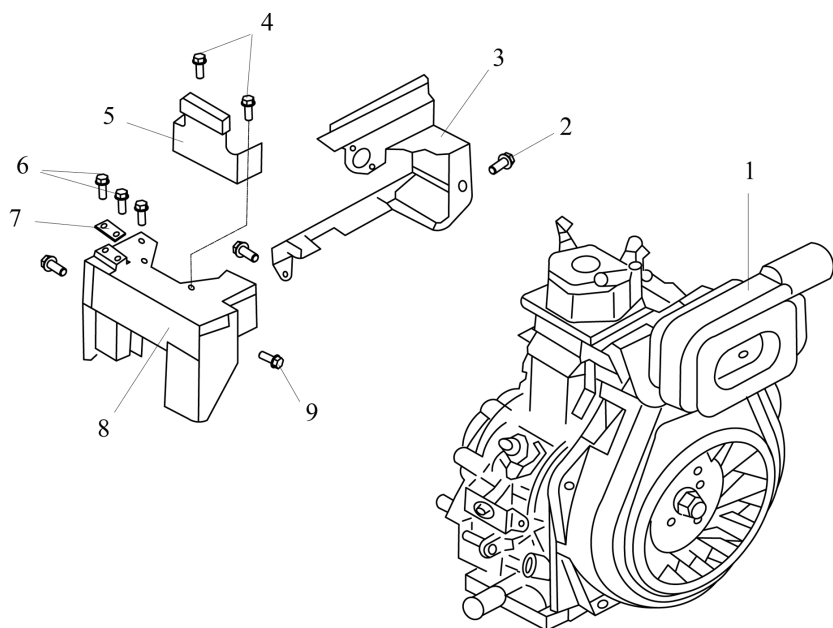
Diesel Engine Assembly
