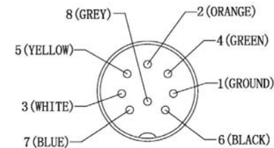
To RO4700 GPS connector
